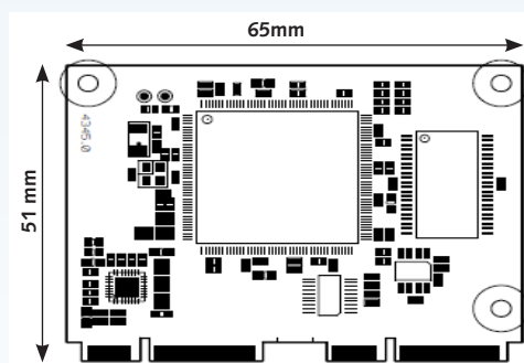
2x52 pin card edge connector (Mini PCIe connector footprint)
